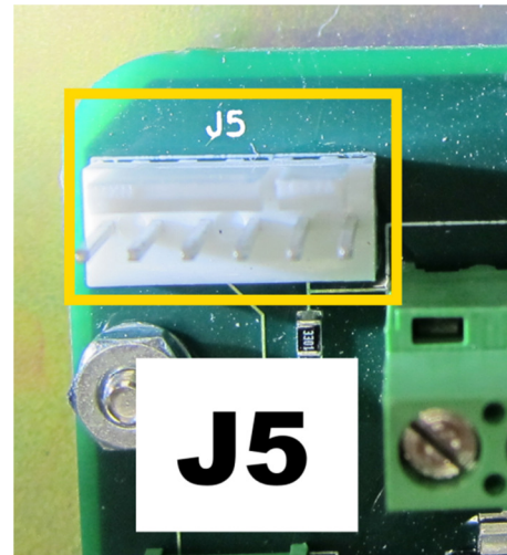
J5 Programming (L->R, 6 5 4 3 2 1)
