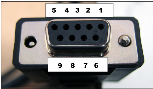
Female Connector Front View, Pre-molded Cable
