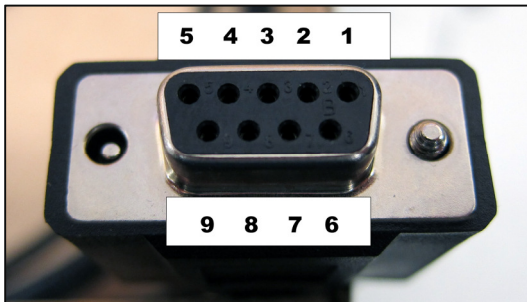
Female Connector Front View
