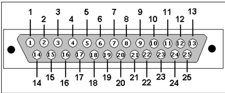
Male Connector Front View
