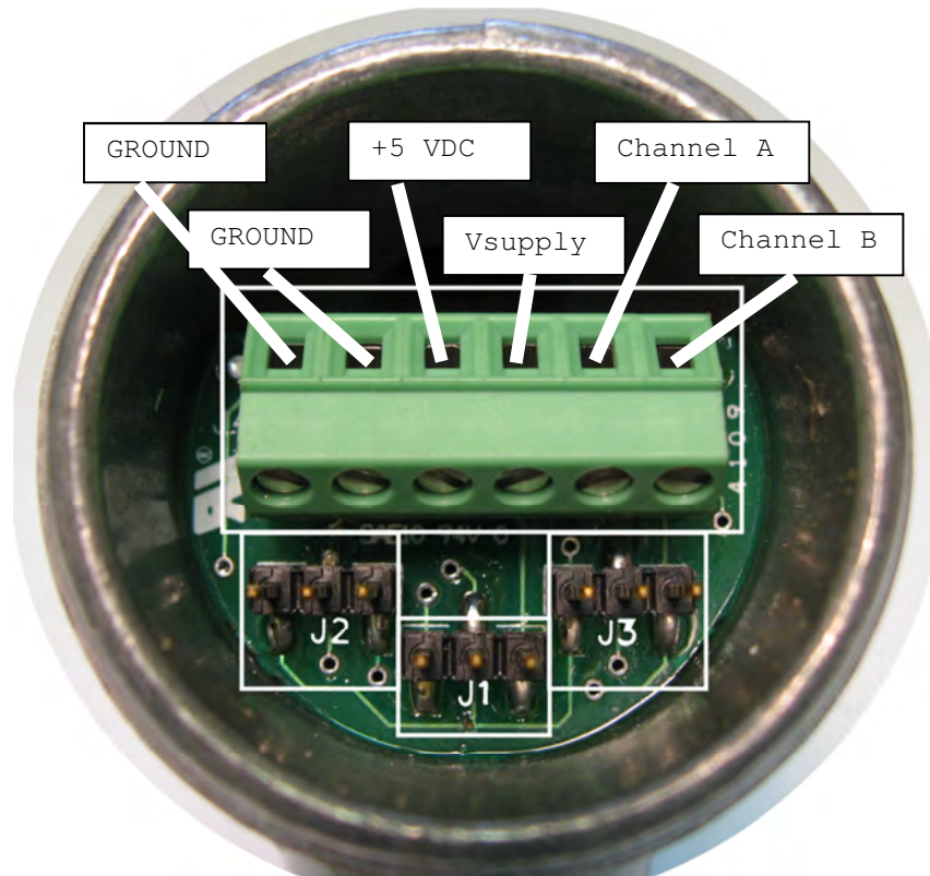
Figure 13. PT-10 REMOTE PULSER CONNECTOR AND JUMPERS
