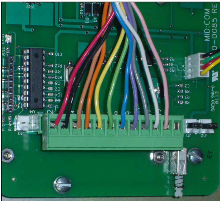
Figure 6. REGISTER CONNECTOR WIRING DETAILS
