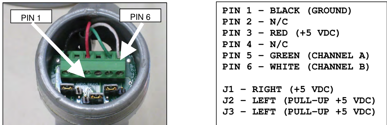
Figure 12. PT-10 REMOTE PULSER LTIS CABLE CONNECTION
