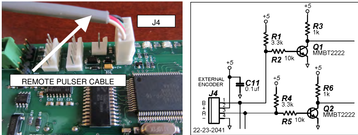
Figure 12. PT-10 REMOTE PULSER LTIS CABLE CONNECTION
