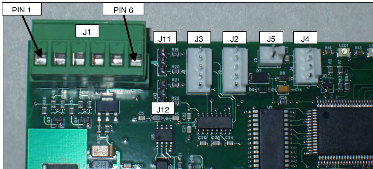
Figure 7. CONTROL BOARD CONNECTION DETAILS
