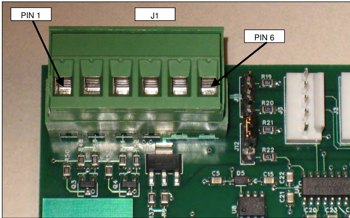
Figure 9. FUEL MANAGEMENT SYSTEM CONNECTOR (J1)
