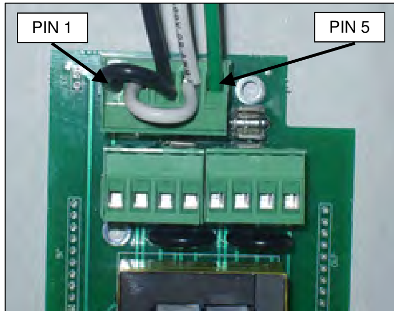
Figure 4. 120 VAC MAINS WIRING DETAILS
