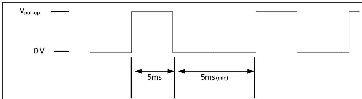
Figure 8. PULSE OUTPUT TIMING DIAGRAM
