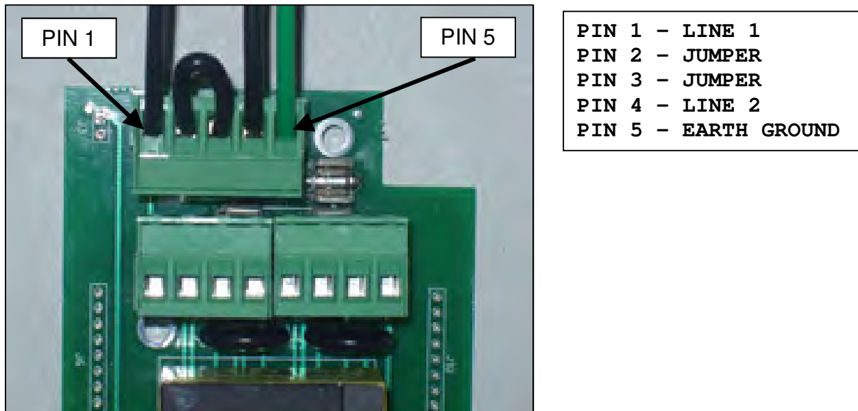
Figure 3. 240 VAC MAINS WIRING DETAILS
