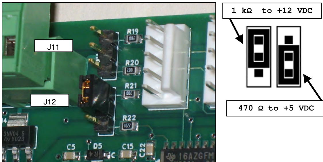
Figure 10. OUTPUT 2 PULLUP JUMPER (J12) SET FOR +12 VDC
