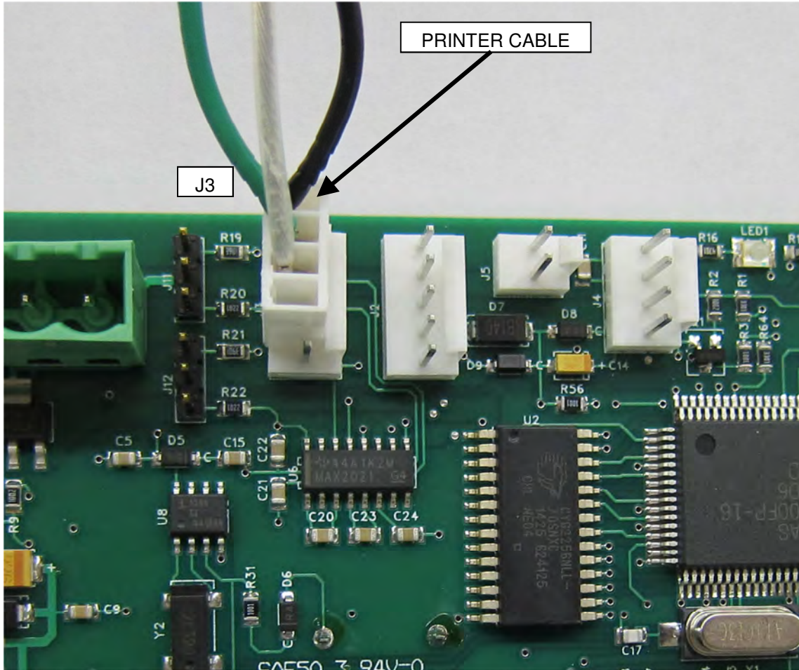
Figure 14. PRINTER WIRING DETAILS (J3)
