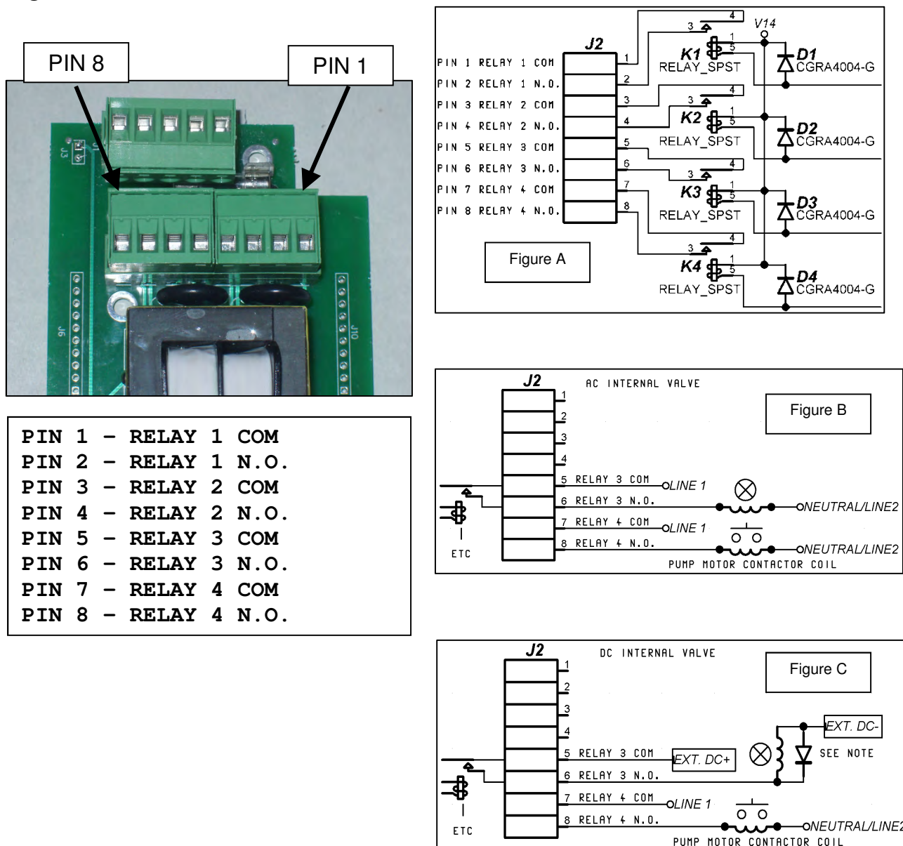
Figure 5. RELAY CONNECTOR WIRING DETAILS
